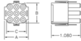
9, 12 AND 15 CIRCUIT
